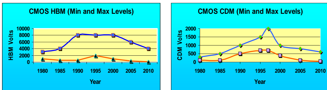
Figure 26. ESD Roadmap for HBM and CDM [12].
