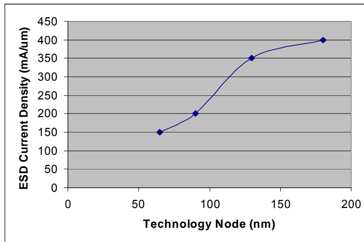
Figure 15. Metal ESD failure current density as a function of technology node.
