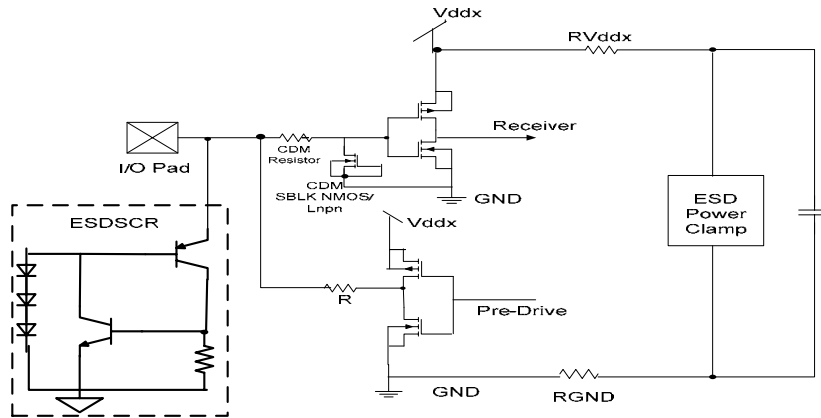
Figure 24. Diode String Triggered SCR (DTSR) with RC-triggered Rail Clamp ESD Protection Strategy
