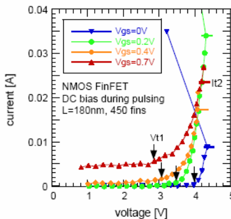
Figure 18. I ds -V ds curves for varying gate bias with trigger voltages (V t1 ) and failure currents (I t2 ) shown for a FinFET device structure [5].
